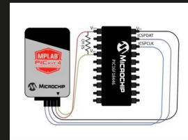
External PICKIT4 JTAG in-circuit programmer/debugger
