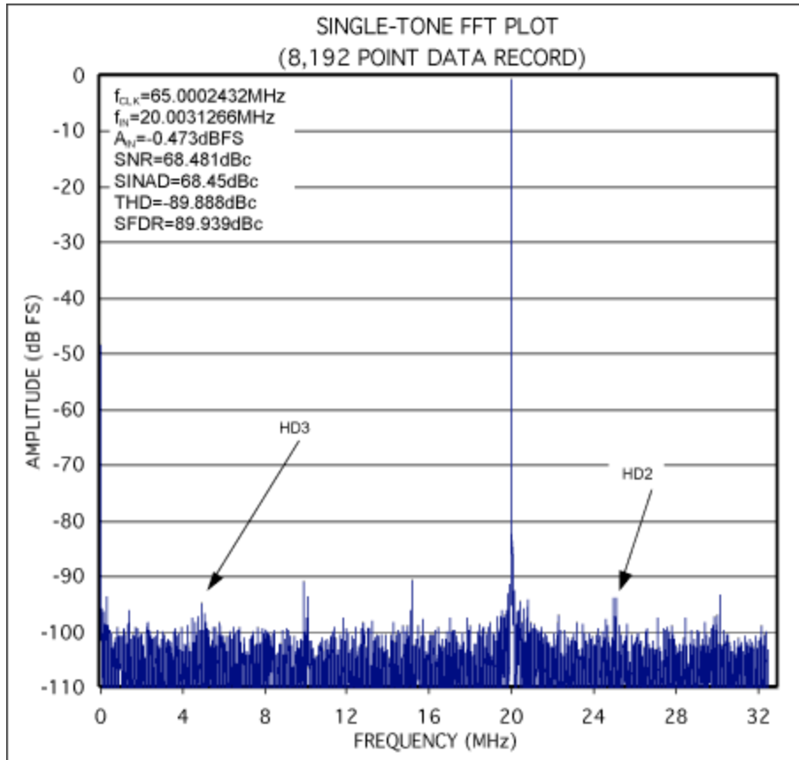
Figure 2. Coherently sampled FFT from the MAX1211EVKIT. f_{CIN}=20.0031266\text{MHz} f_{CSAMPLE}=65.0002432\text{MHz} N_{WINDOW}=2521 N_{RECORD}=8192
