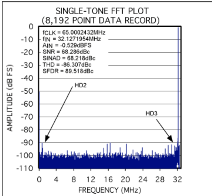
Figure 3. Coherently sampled FFT from the MAX1211EVKIT. f_{CIN}=32.1271954\text{MHz} f_{CSAMPLE}=65.0002432\text{MHz} N_{CWINDOW}=4049 N_{RECORD}=8192
